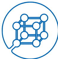
Compounds
