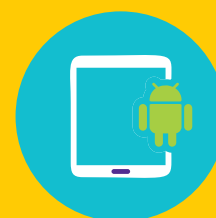
Android Application
