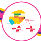
Functional Genomics
