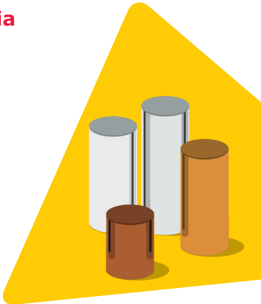
Compounds
